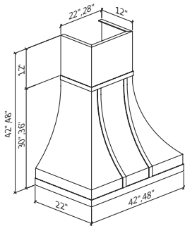
METAL HOOD (WIDTH: 42-48)
