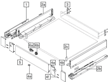
BID-M BID-M: Blum Inner Draw-M
