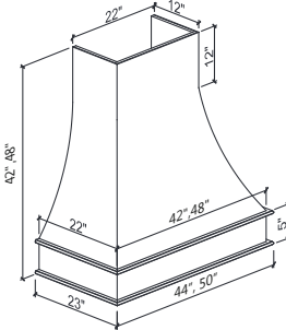
WOOD HOOD B (WIDTH: 44-50)
