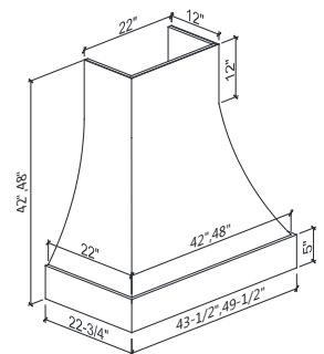
WOOD HOOD A (WIDTH: 43-1/2-49-1/2)
